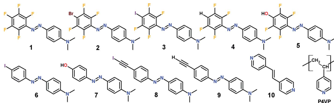
Fig. 1 Chemical structures of fluorinated azobenzene modules 1–5, hydrogenated azobenzene modules 6–9, model dipyriddy compound 10 used in the co-crystallization studies, and poly(4-vinyl pyridine) (P4VP) that was used as the polymer matrix for the azobenzene dyes.
