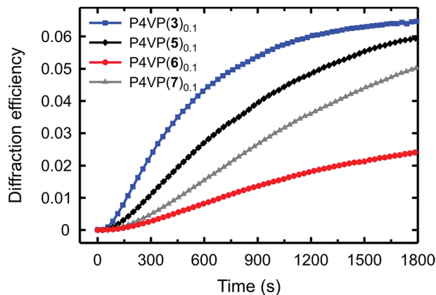
Fig. 5 Kinetics of the first-order diffraction efficiency upon the grating inscription process for P4VP( n ) 0.1 , where n = 3 ( l is para to the azo group), 5 (OH is in the para position), 6 ( l is in the para position on a non-fluorinated ring), and 7 (OH is in the para position on a non-fluorinated ring).
